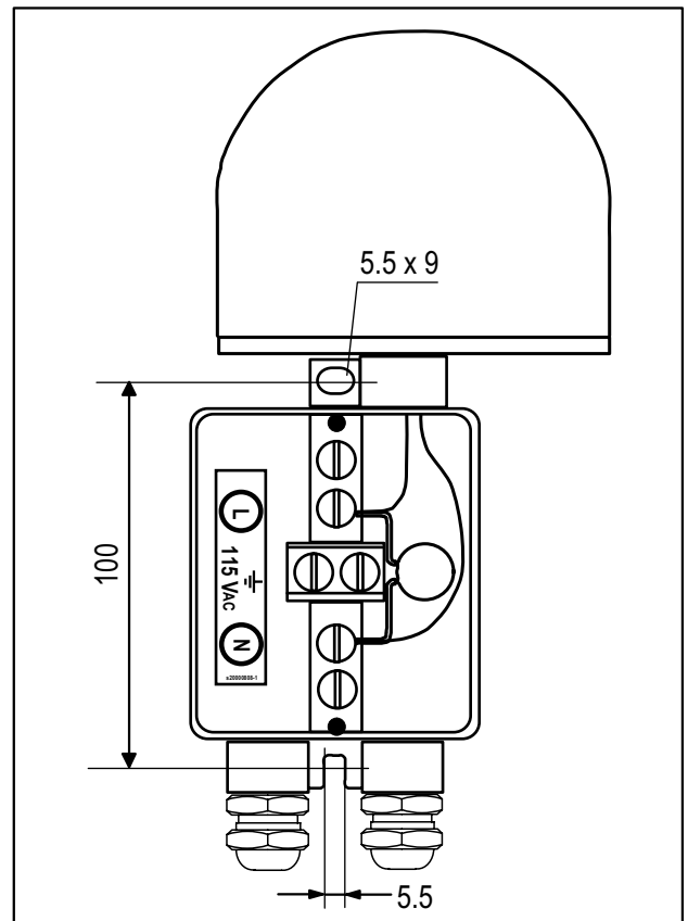
Obelux 10-115-F terminal box
